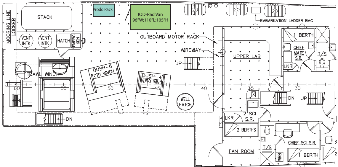
R/V New Horizon 01 Deck Plan General CalCOFI Setup
